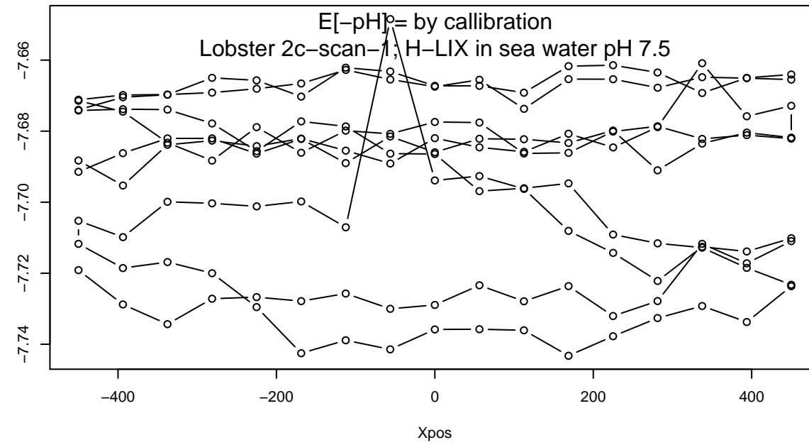
scatterplot3d - L
