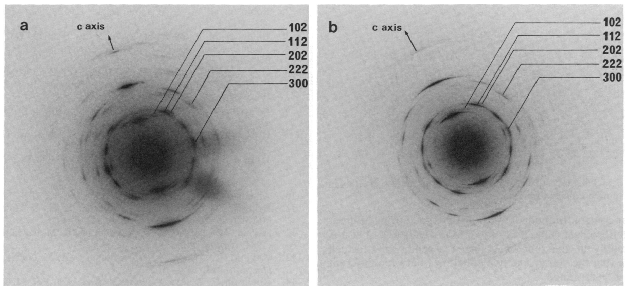
FIG. 5. Electron diffraction patterns of longitudinal sections of mineralized turkey tendon. (a) Diffraction from selected area of 0.3- \mu\text{m} diameter. This pattern shows h o l -type reflections (e.g., 300, 102, and 202) relatively intense compared with h h l -type reflections (e.g., 112, 222), in contrast to that of b , indicating well-defined orientation of apatite crystallites with their b axes lined up with the electron beam. (b) Diffraction from selected area of 0.9- \mu\text{m} diameter, corresponding to most of the region shown in Fig. 4a. This pattern shows h h l -type reflections, including 112 and 222, relatively intense compared with h o l -type reflections, such as 300, 102, and 202. This indicates a nearly uniform orientation of the crystallites with their 100 faces perpendicular to the electron beam and tilted some 30^\circ about their c -axis directions from the orientation of Fig. 5a. Some distortions were evidently introduced into the specimens during sample preparation, so the best areas were sought. As shown here, well-oriented and balanced diffraction patterns corresponded to well-ordered banding patterns in electron micrographs. However, diffraction proved the more sensitive criterion, so regions for data collection were sought first in the "image" and then in the "diffraction" mode of the electron microscope.
