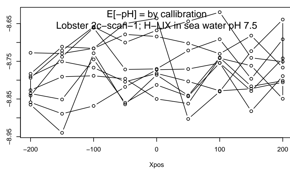
scatterplot3d - L
