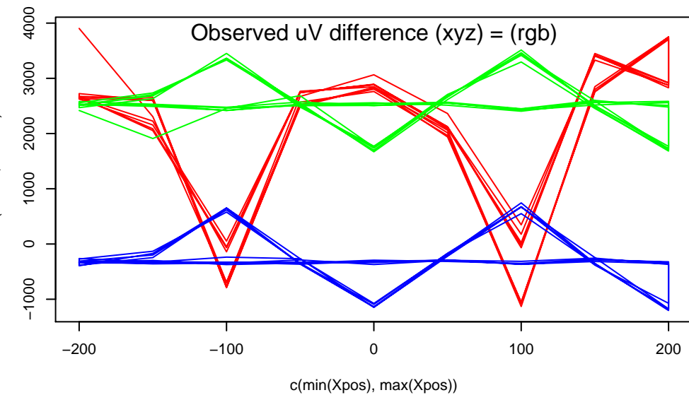
Lobster016.TXT Obs[uVdiff]
