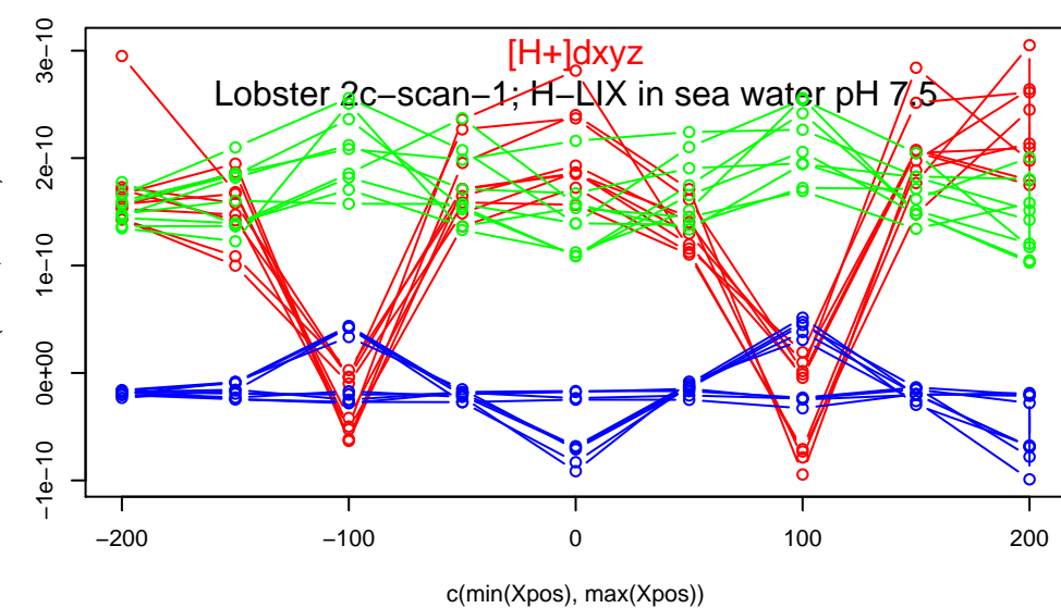
Lobster016.TXT [H+]dxyz
