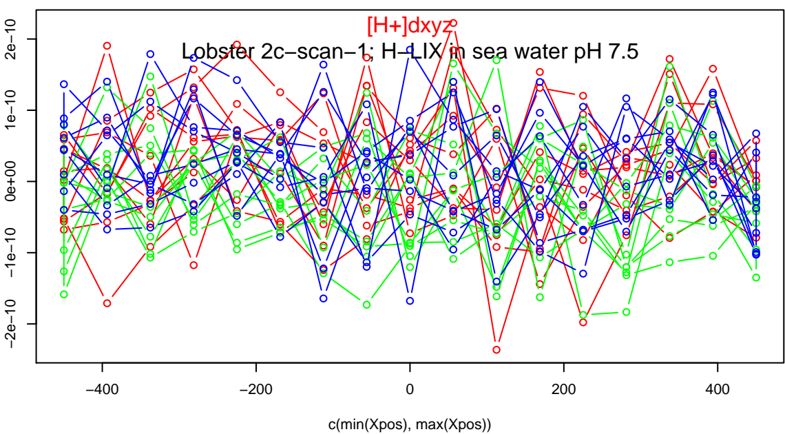
Lobster009.TXT [H+]dxyz
