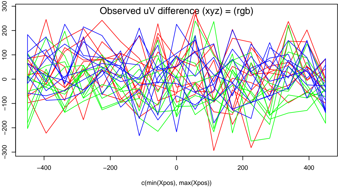
Lobster009.TXT Obs[uVdiff]
