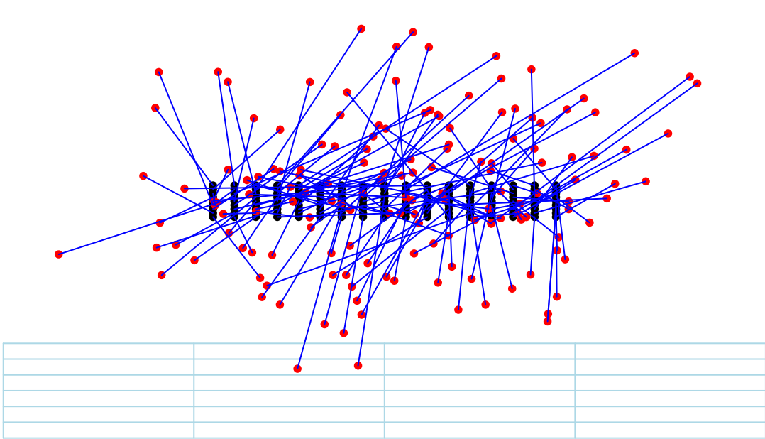
scatterplot3d - R
