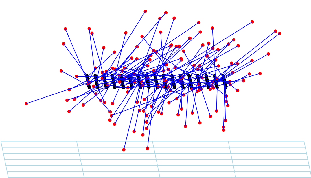
scatterplot3d - L
