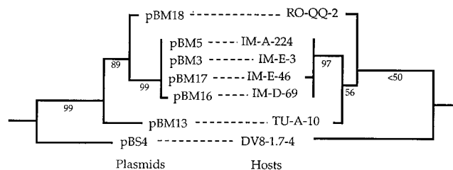
FIG. 2. Comparison of the phylogeny of plasmids from size group 1 with the phylogeny of their host strains. The phylogeny of these plasmids was rooted by using plasmids from size group 2 (plasmids pBM11, pBM14, and pBM15) as an out-group; the phylogeny of strains was rooted by using strain DV8-1.7-4 as an out-group. The percentages of bootstrap support greater than 50% are shown. Dashed lines connect plasmids with their host strains.
